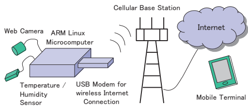
Figure 1 System configuration
