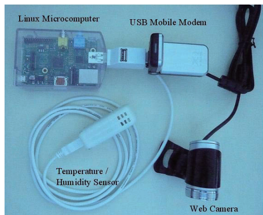
Figure 2 System configuration
